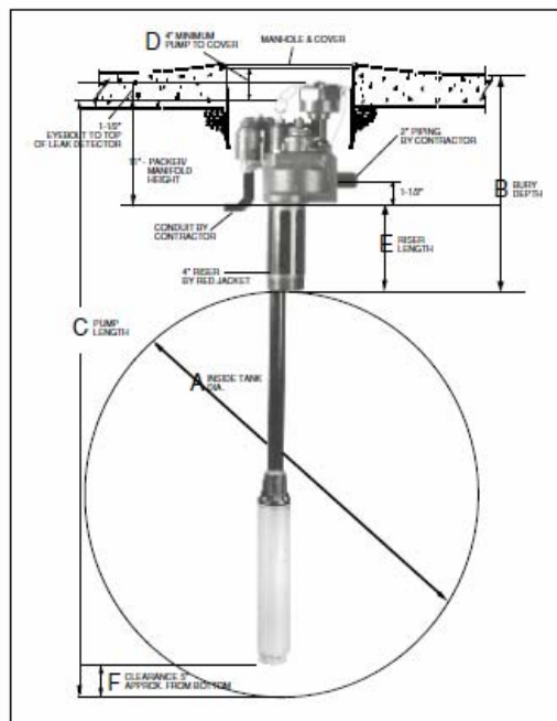
FIGURE 1: 4" Submersible Pump mounted in a single wall tank
